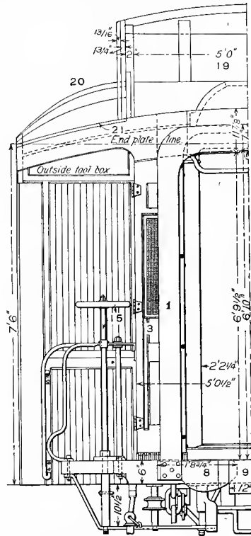
Fig. 2426. End Elevation.
